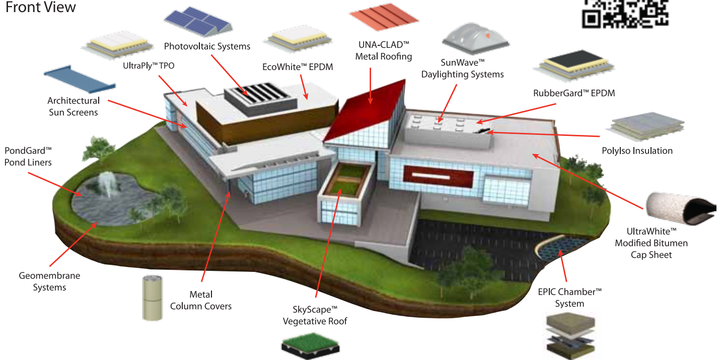
Front View
