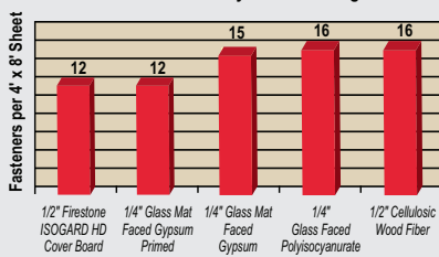
Fastener Density for I-90 Rating
