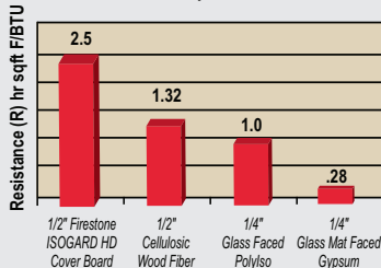
R-Value per Thickness
