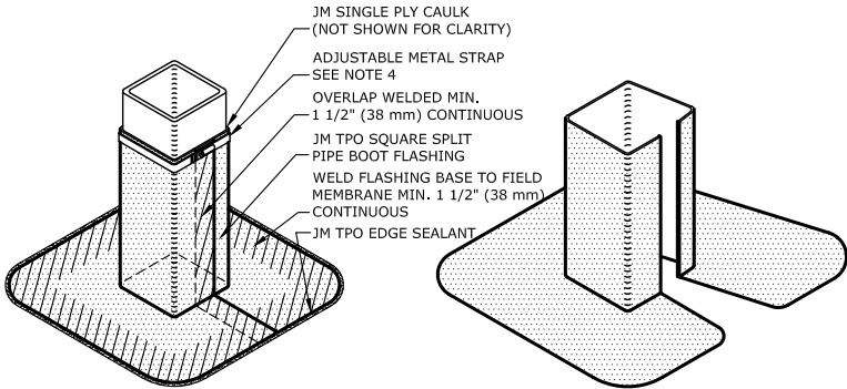
INSTALLED BOOT ISOMETRIC VIEW
