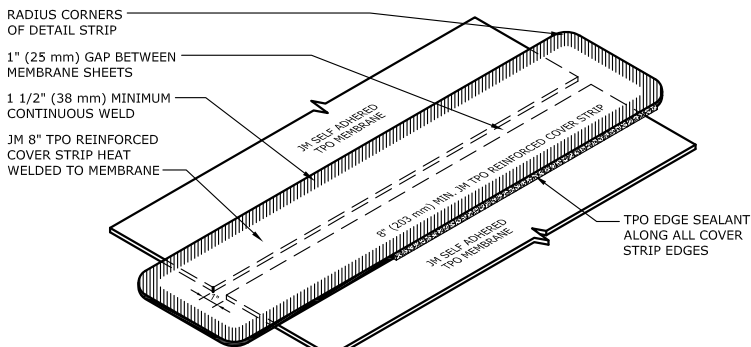
ISOMETRIC VIEW
