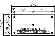
INSULATION FASTENING
