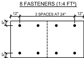
FIELD
