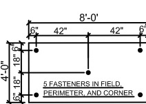
INSULATION FASTENING
