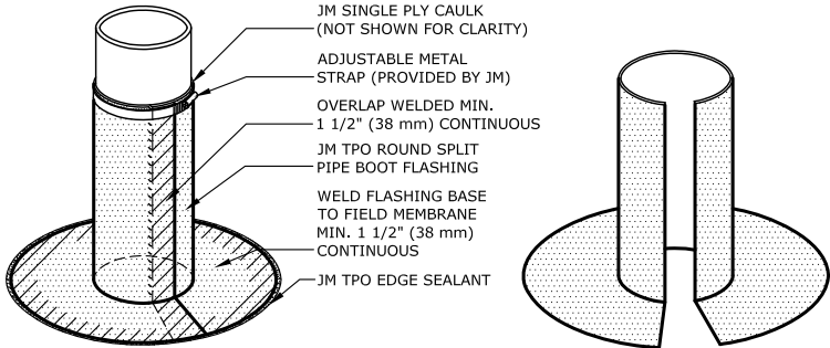
INSTALLED BOOT ISOMETRIC VIEW
