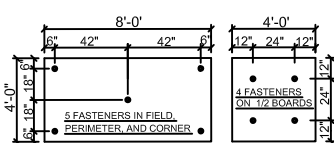
INSULATION FASTENING
