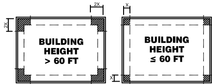
CORNER DEFINITION
