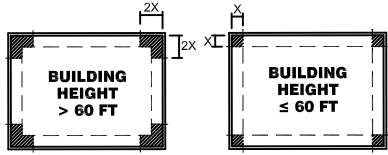
(SEE NOTES 5 & 6) CORNER DEFINITION
