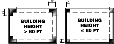
CORNER DEFINITION
