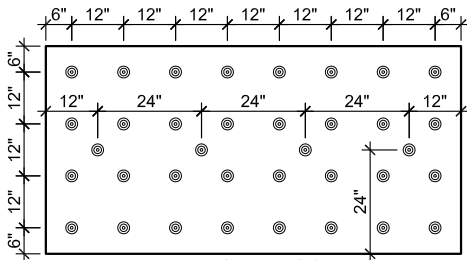
36 FASTENERS / BD.
