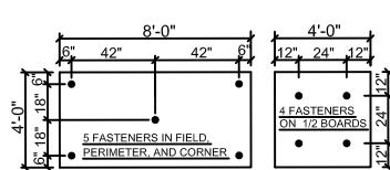
INSULATION FASTENING
