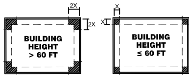
CORNER DEFINITION
