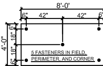
INSULATION FASTENING
