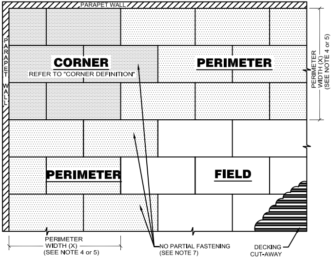
8 FASTENERS (1:4 FT 2 )
