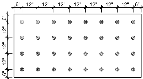
32 FASTENERS / BD.
