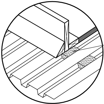
ISOMETRIC VIEW OF STEEL DECK INSTALLATION
